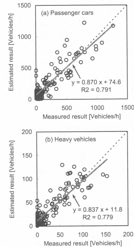
Figure 7. Comparison between estimated and measured traffic volumes
