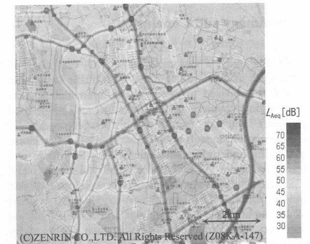
Figure 8. Estimated result of citywide road traffic noise
