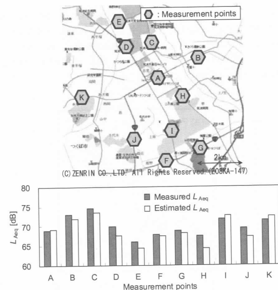
Figure 9. Comparison between estimated and measured L_{Aeq}
