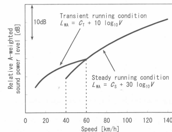
Figure 2. Road vehicles' sound power calculation model of ASJ RTN-Model 2003 [11]
