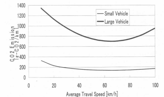
Figure 3. CO 2 Emission Model used in the study
