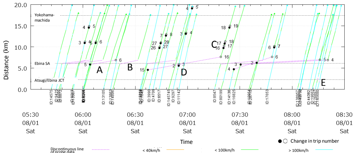
Figure 1: Vehicle trajectories in time-space diagram taken near Ebina SA on the Tomei Expressway (1 August 2015)
