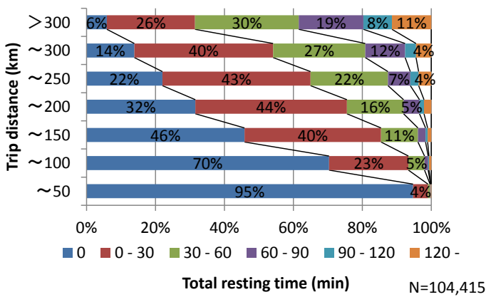
Figure 9: Distribution of resting time (small cars)
