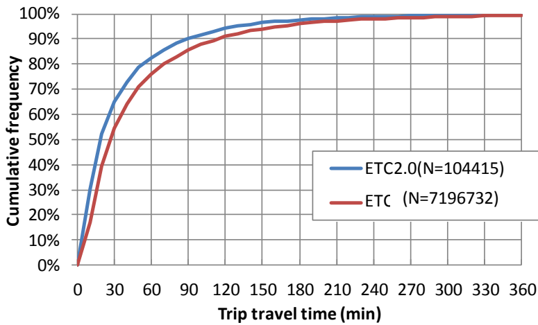
Figure 4: Trip travel time distribution of trip behaviour (small cars)
