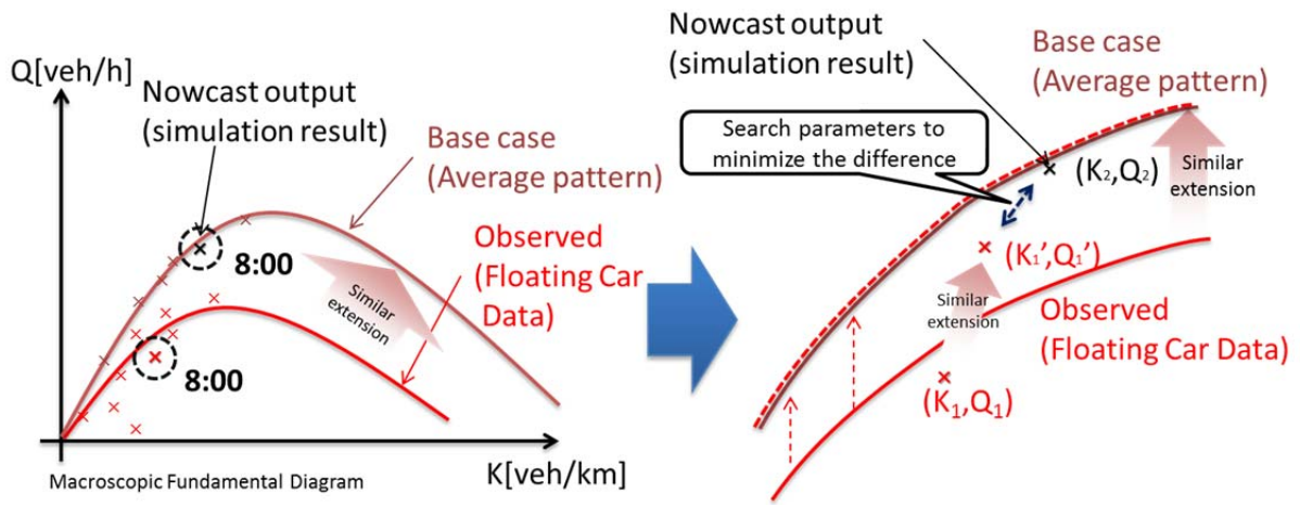
Figure 3: Concept of the evaluation using MFD
