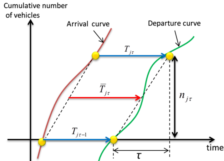
Figure 5: Cumulative curve to calculate an average link travel time
