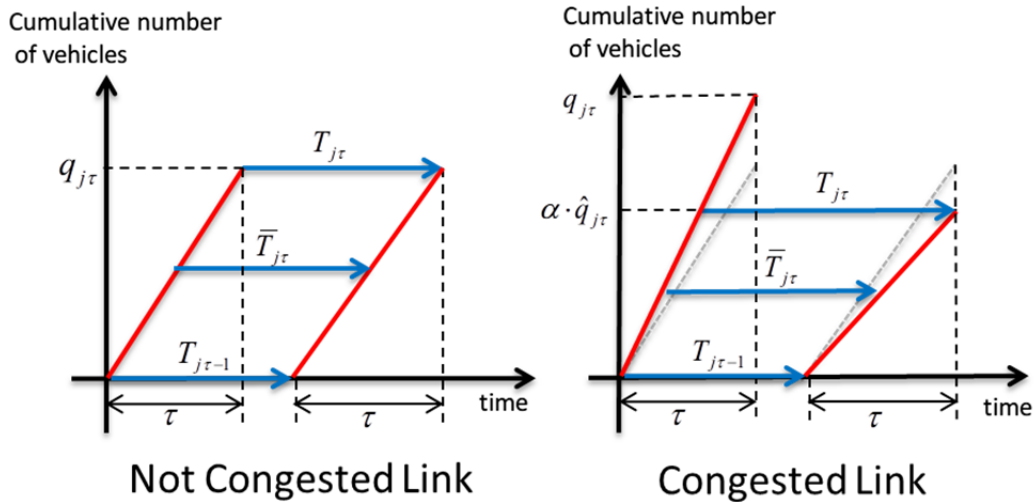
Figure 6: Variation of cumulative vehicle count curves
